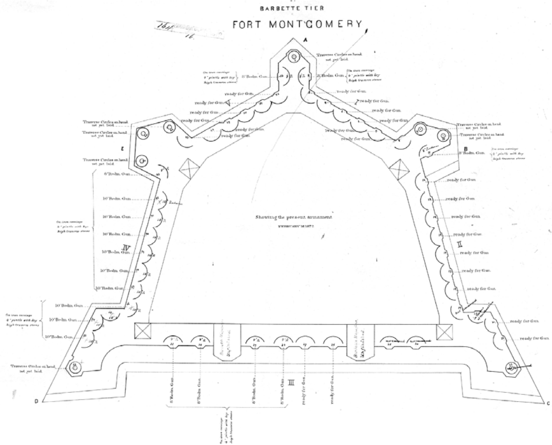
Armament of the barbette tier, February 1872. NARA, Drawer 259, Sheet 95
